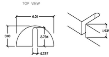
MOUNTING SLOT DETAIL SCALE 2:1 ALL DIMS NOMINAL
