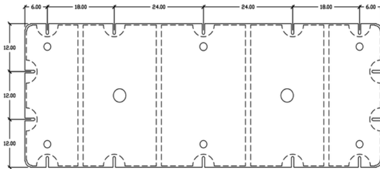
MOUNTING SLOT DETAIL SCALE 2:1 ALL DIMS NOMINAL
