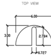
MOUNTING SLOT DETAIL SCALE 2:1 ALL DIMS NOMINAL
