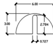
MOUNTING SLOT DETAIL SCALE 2:1 ALL DIMS NOMINAL
